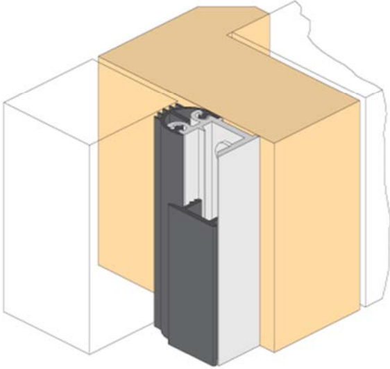
RP10 perimeter seal
