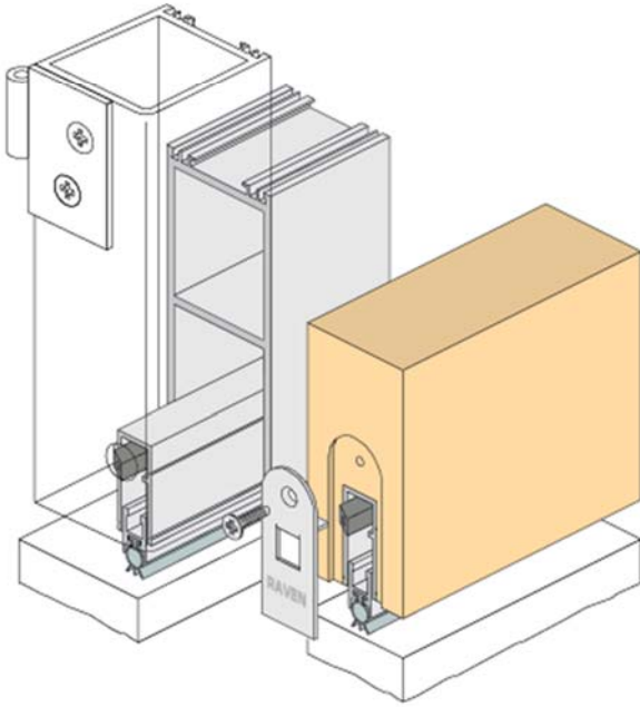
RP8 mortise drop seal
