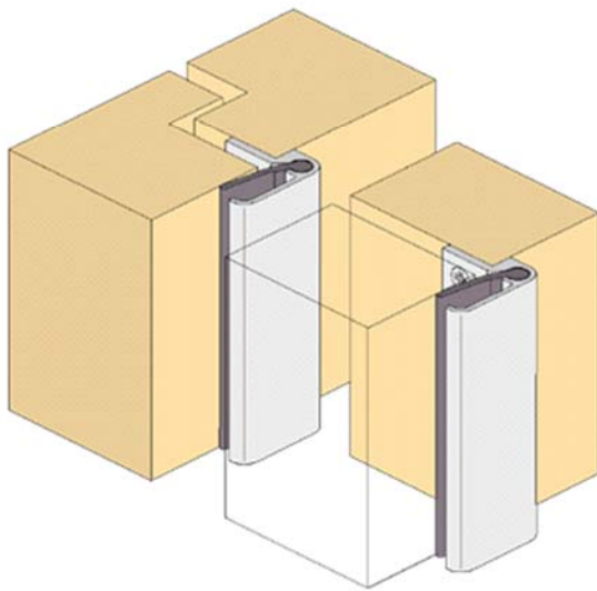
RP16 double door seal
