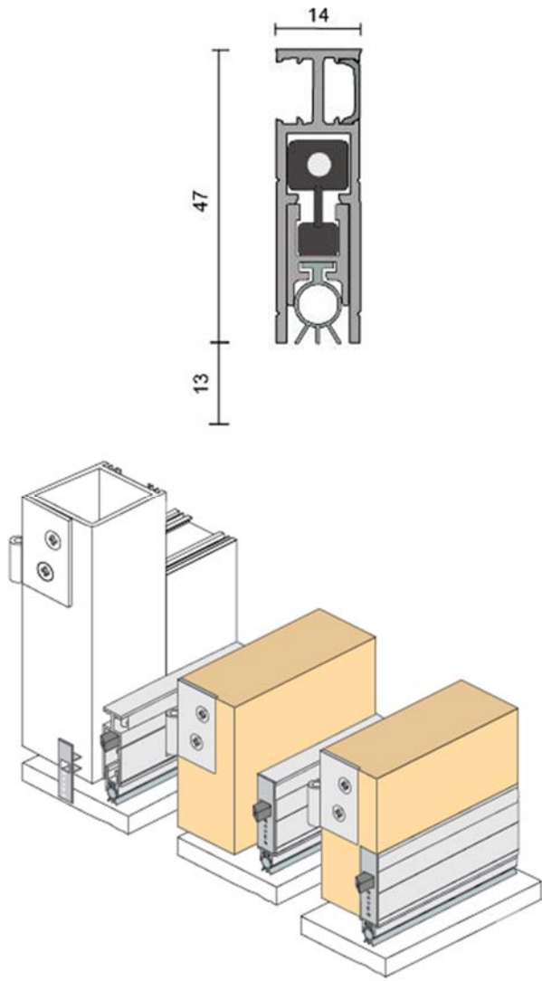
RP35 face fix drop
